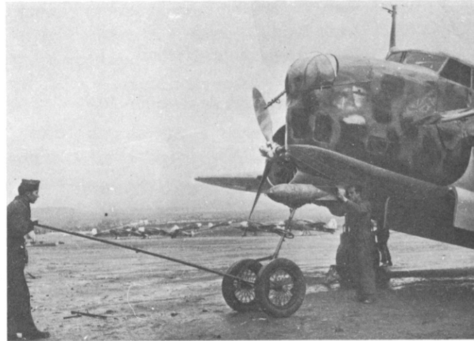
41. A rudimentary bomb hoist is employed for the arming of a Fiat BR 20 bomber of the 35° Gruppo Autonomo Misto at Tablada airfield. In the background can be seen a variety of aircraft including several Caproni Ca 310 twin-engined light bomber-reconnaissance aircraft, which were supplied to the Nationalists late in the war. (Nicola Malizia)
