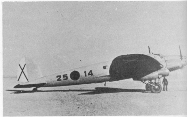
31. Heinkel He 111B of the Legion Condor . These aircraft were later handed to the Nationalists after more modern E models had arrived from Germany for K/88 . The first Spanish He 111 unit, 10-G-25 , went into action during the Battle of the Ebro in August 1938. (Franz Selinger)
