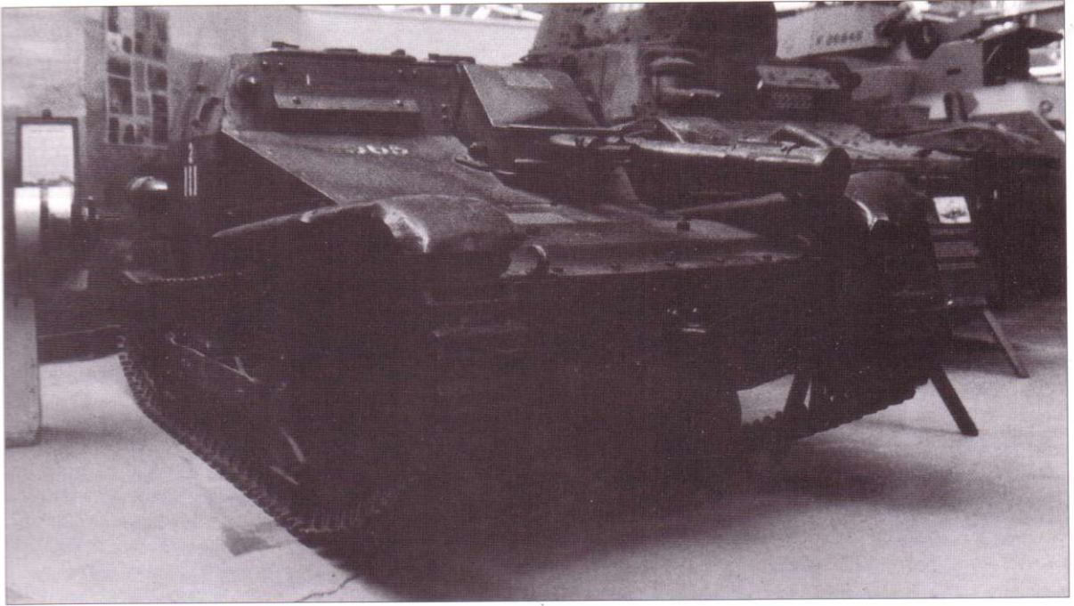
CV33 Lanzallamas. This is the flame thrower version of the CV33 tankette, of which several examples were sent to Spain. Although not up to the task of armoured warfare because of poor armament and armour, they were employed as tractors and machine gun carriers right up to the end of the war. (RAC Museum)
