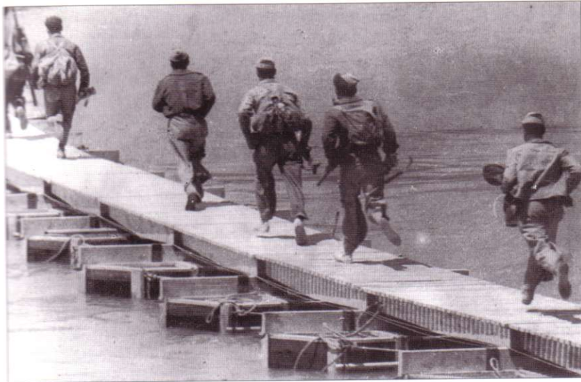
One of the puentes de corcho or pasarelas ; the light foot bridges used to cross the River Ebro. Hexagonal cork floats were positioned every 2.5 metres along their length for stability. It was theoretically possible to transfer 3,000 men an hour across these constructions. (IWM)
