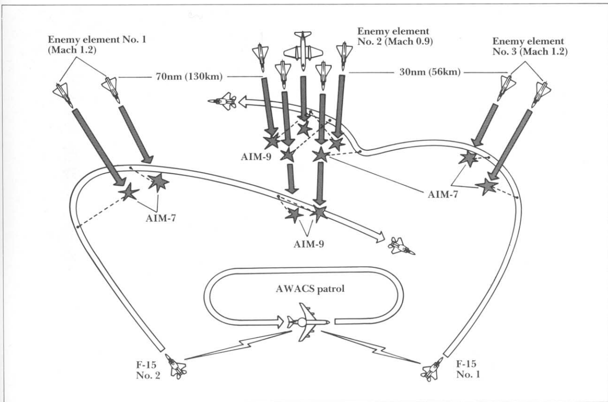
Above: Despite being outnumbered nine to two, when working in conjunction with an E-3 Sentry, the F-15 should theoretically emerge victorious by destroying adversaries at long-range with the Sparrow and then using Sidewinder to mop up the remnants. This exercise, conducted on an instrumented range at Yuma, Arizona, resulted in destruction of all nine "targets".
