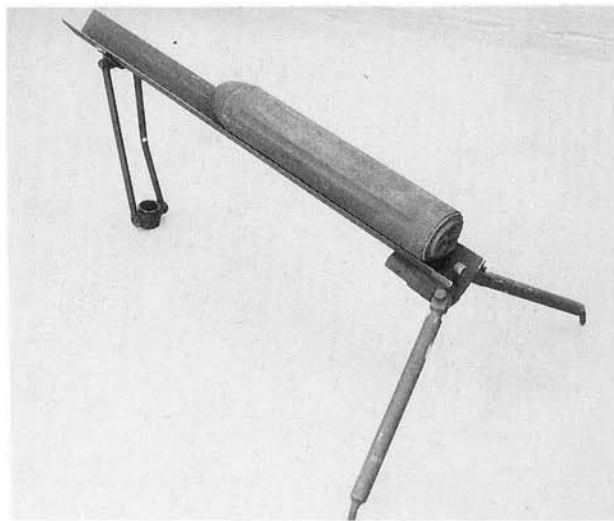
A 9-pdr. Hales rocket trough, used in Zululand. One arm of the trough is missing, and this rocket seems to be a larger 24-pdr. type. (Natal Museum)
