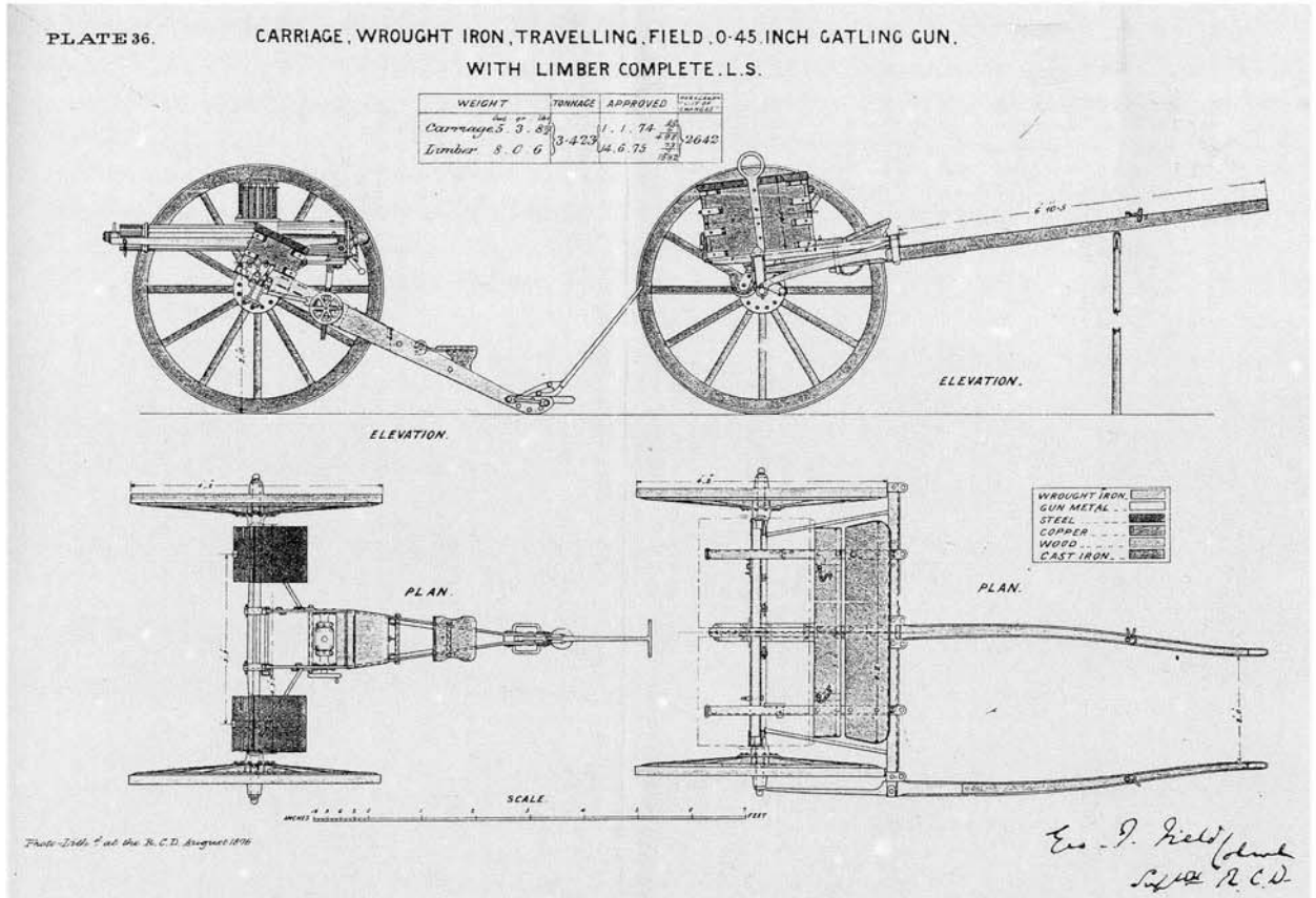
Plans of the .45in. Royal Artillery Gatling, its carriage and limber (Royal Artillery Institute, Woolwich)
