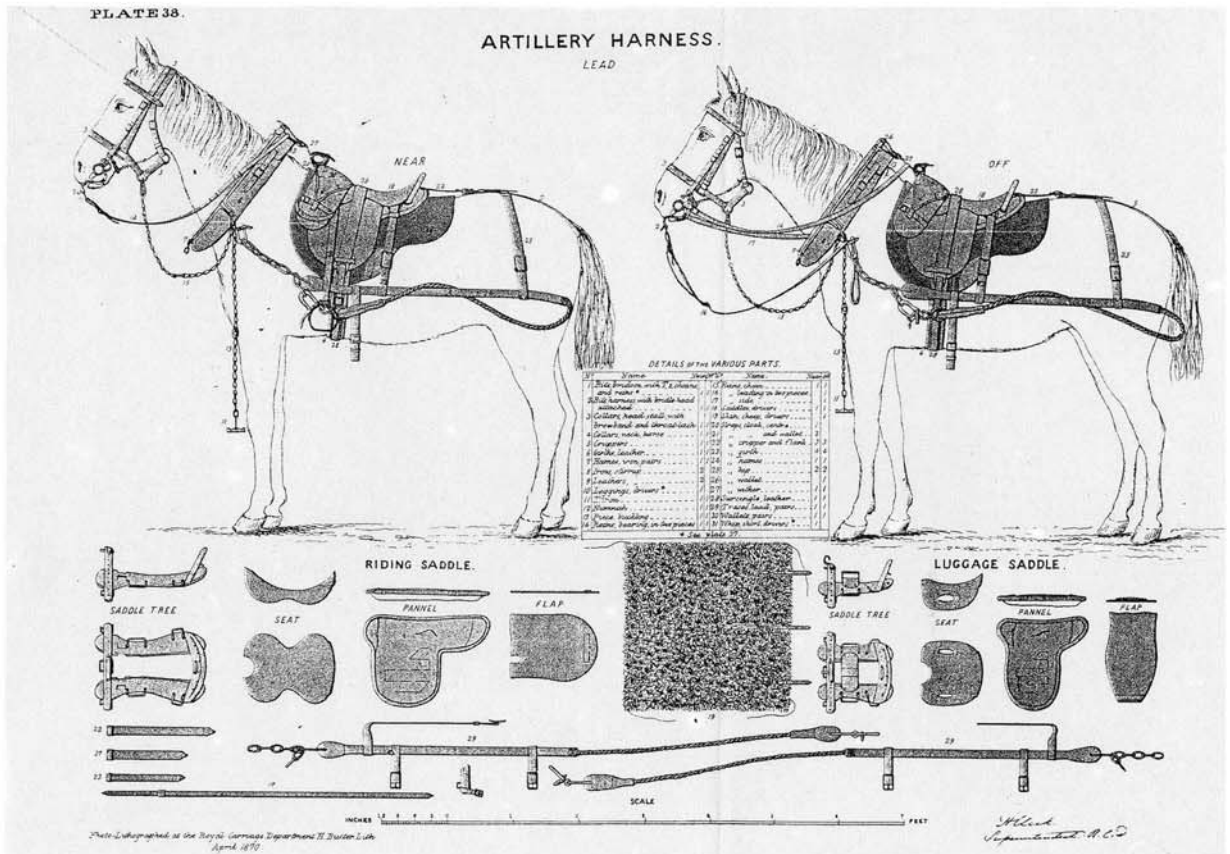
Details of the harness equipment used to pull the 16-pdr. RML limber. (Royal Artillery Institute, Woolwich)
