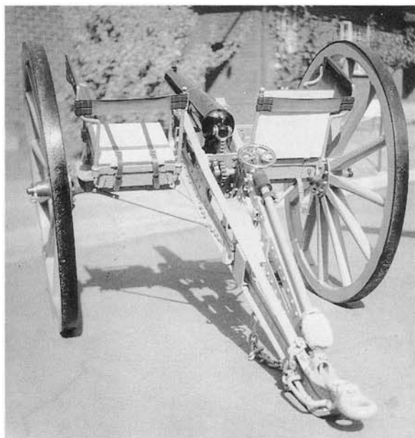
A 7-pdr. RML gun used in the Zulu War, mounted on a 'Kaffrarian' carriage, a modified version of the 9-pdr. carriage. (SA Museum of Military History, Johannesburg).
