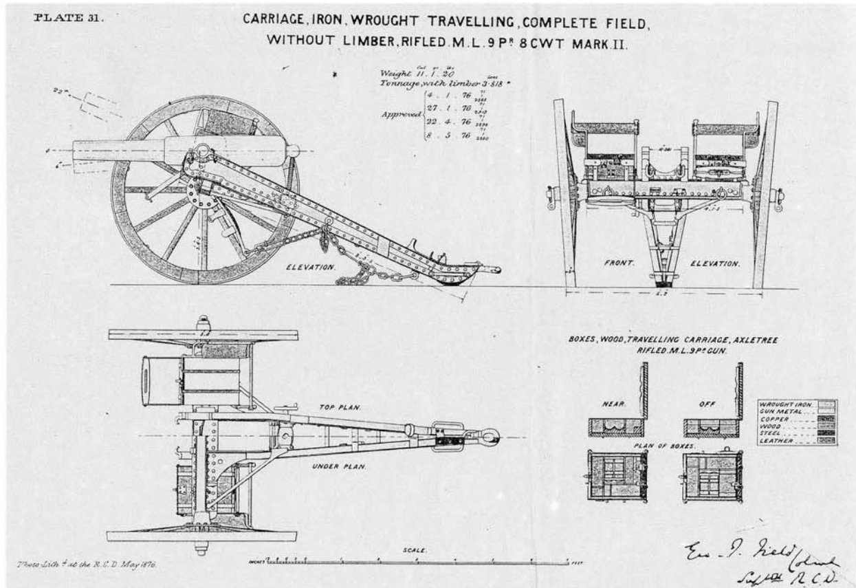
Plan of the 9-pdr. RML gun and its carriage, the standard field piece of the Zulu War. The 7-pdr. RML was sometimes mounted on 9-pdr. carriages with very little modification. (Royal Artillery Institute, Woolwich)
