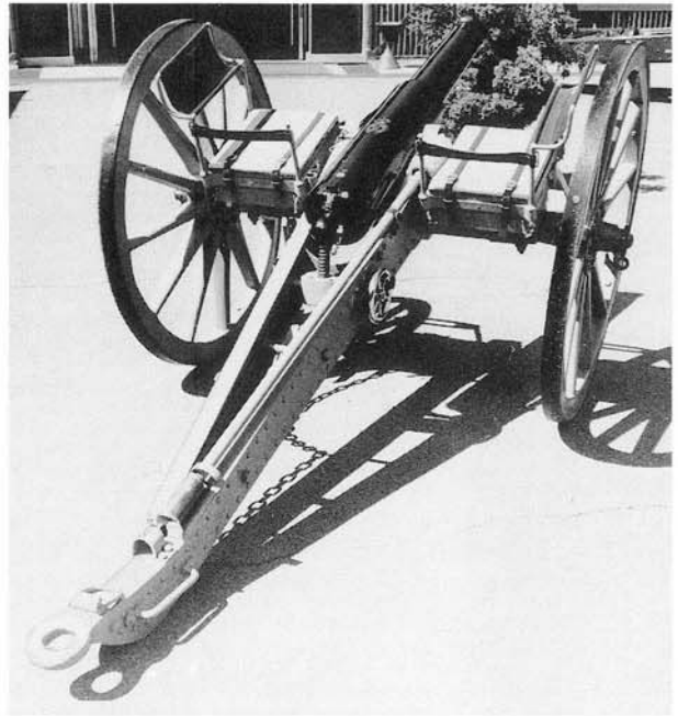
A 9-pdr. RML gun used in the Zulu War. (SA Museum of Military History, Johannesburg).
