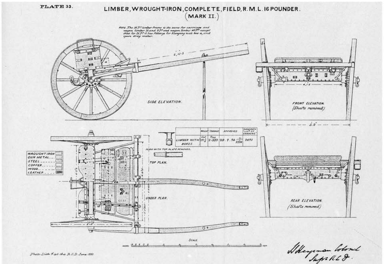
The 16-pdr. RML limber, used in Zululand to pull the 9-pdr. RML. (Royal Artillery Institute, Woolwich)
