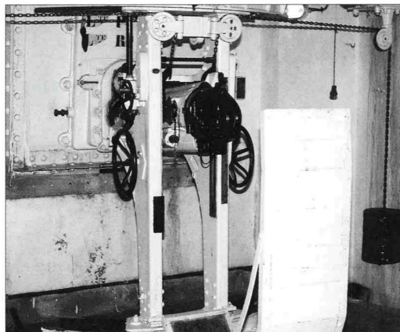
One of the two M1931 75mm 'mortars' of block 2 of the gros ouvrage of L'Agaisen. Unique to the Alps, the 75mm 'mortar' was actually a lightweight howitzer. The counterweight on the right is one of two that supports the breech of the gun. (Author's photograph)
