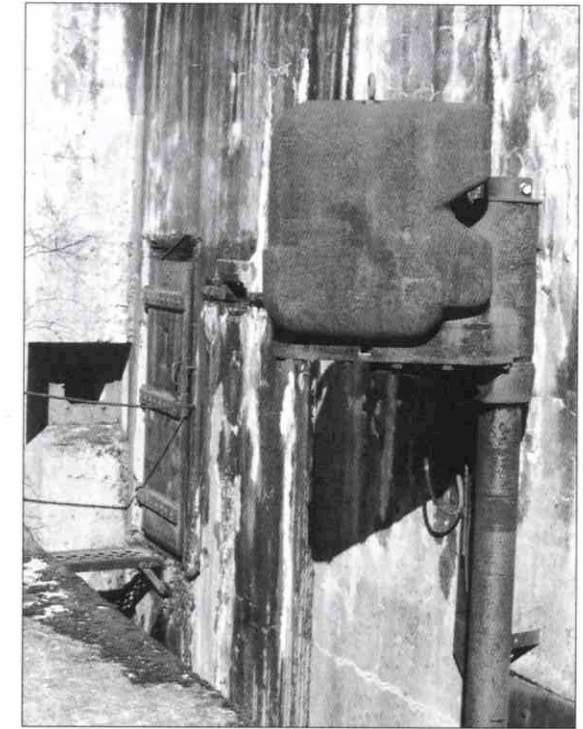
The rear of the interval casemate of Veckring North. In the background is the embrasure for the automatic rifle protecting the casemate's entrance and the entrance itself. In the foreground is the casemate's armoured searchlight. (Author's photograph)
