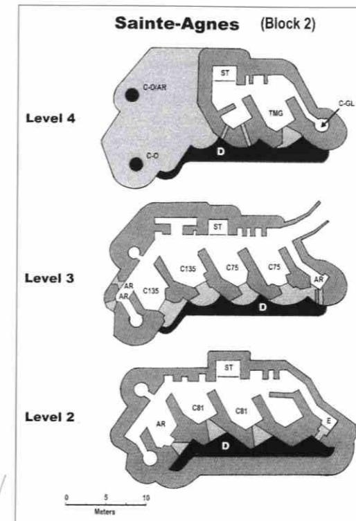
ABOVE RIGHT Block 2 of the gros ouvrage of Sainte-Agnès is generally accepted to be the most heavily armed combat block in the entire Maginot Line programme. It is spectacularly sited overlooking the town of Menton and fires over the town toward the Mediterranean Sea. The two 75mm weapons are 75mm 'mortars'. Not shown in the plan is the block's lowest level, which contains the machinery for the lift that transports ammunition to the other levels. (Eric Halter/John Richards)
