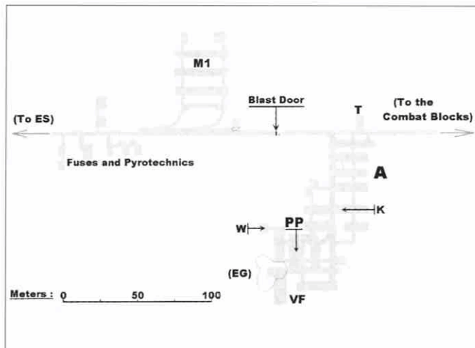
A fairly typical support area for the Soetrich gros oufrage in north-eastern France. The oufrage's 0.6m gauge electric railway runs along the main gallery. (Eric Halter)
