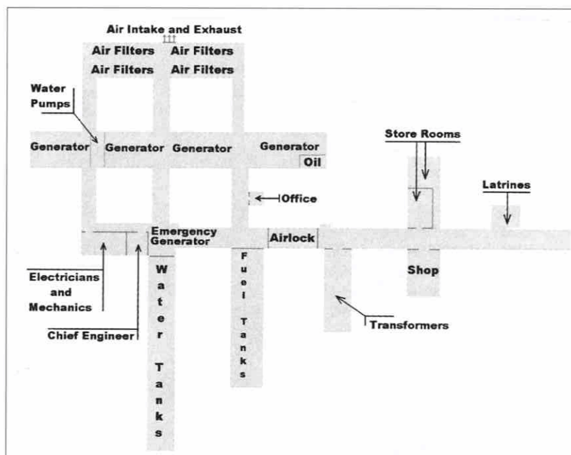
The power plant area of the gros oufrage of Schoenenbourg, a medium-sized gros oufrage in north-eastern France. Each of the four diesel-engine-powered generator sets was capable of producing 160 kW of 440 volt, 50 cycle, alternating current. Most electrical equipment within the oufrage operated at 440 volts, but the power plant contained the converters and transformers necessary to produce the 600 volt direct current required by the railway locomotives and the 120 volt direct current required by the turret motors. The power plant could also convert high-voltage current provided by the national power grid to meet the oufrage's needs. (Eric Halter)
