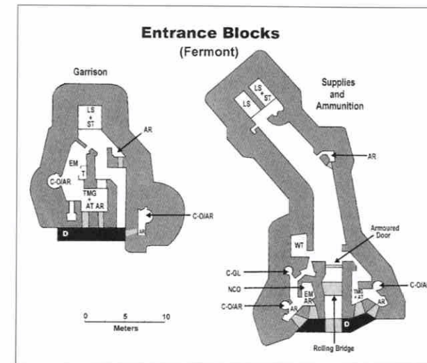
Ground level plans of typical entrance blocks for a gros oufrage in north-eastern France. In this oufrage , descent to the gallery level is by means of vertical shafts. In the supplies and ammunition entrance block, one shaft is equipped with a 5 tonne lift while the other is equipped with a 2.5 tonne lift and a staircase of 96 steps. The garrison entrance block shaft has a 2.5 tonne lift and staircase of 124 steps. Both blocks have lower levels housing equipment and limited accommodation for the block garrison. (Eric Halter/John Richards)
