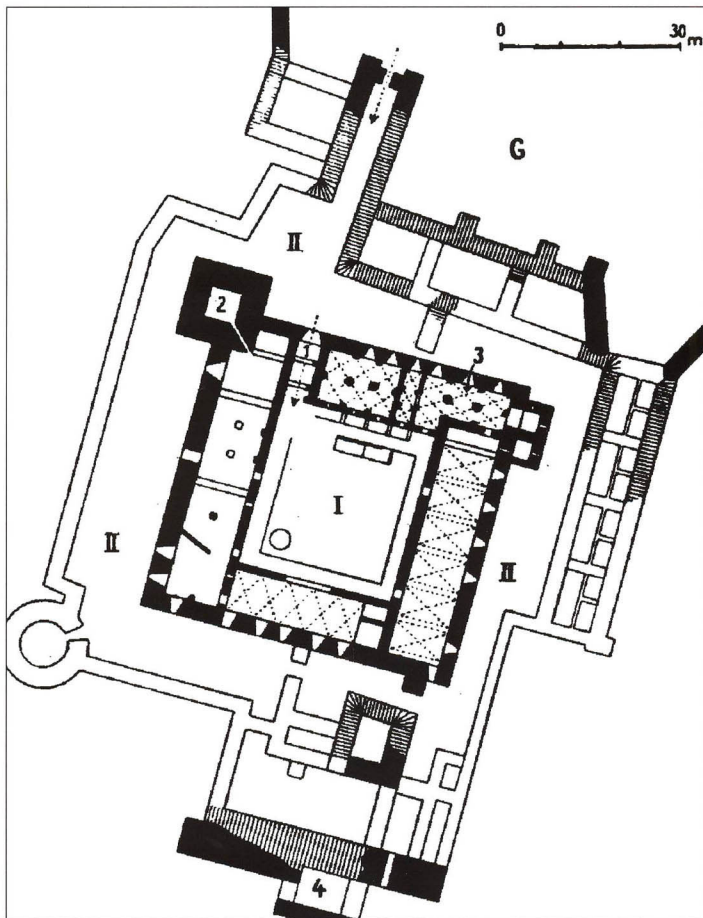
The convent building of Fellin (Viljandi). Ground-floor plan of the structure that fitted into the area described above.
