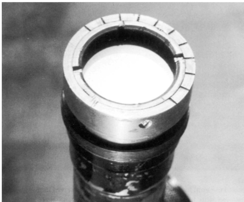
The objective lens of the Aldis scope. To adjust for windage, a brass cover first had to be unscrewed to expose the three tiny grub screws, one of which is visible in the photo. These had to be loosened and a special key was then inserted into the two slots on the lens collar. Turning fractionally left or right altered the position of the vertical aiming post in the graticule. It was a slow and very fiddly affair (Author's collection)
