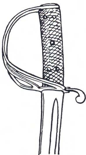
Hilt of trooper's sword, 1853. Described in Army Order 1854 as 'a new sword, essentially a thrusting weapon', the trooper's sword has a straight blade 35 in. long with a spear-point. The grip is of two thick pieces of leather chequered and riveted on either side of the tang, and the guard is of the three-bar type – unfortunately providing rather weak protection to the hand
