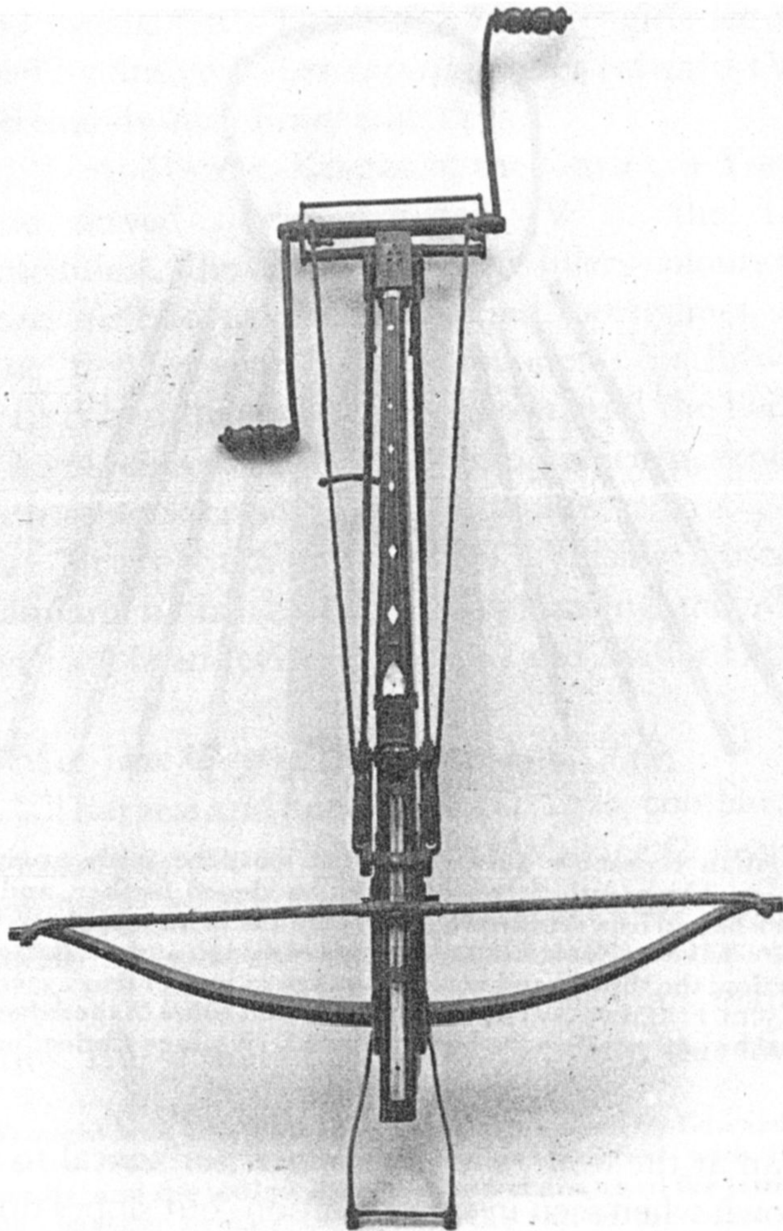
This crossbow, with a steel stave, is 16th century, but is relevant in showing the loading windlass in place. The 'stirrup' foot braces were sometimes, as in this case, two iron rods with a leather strap. (Castle Museum, York)
