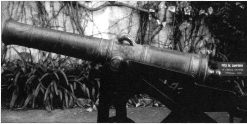
Portuguese brass 9-pdr cannon. The markings indicate it was cast at Lisbon's 'Arcenal Real do Exercito 1802'. (Museu Militar do Porto)
