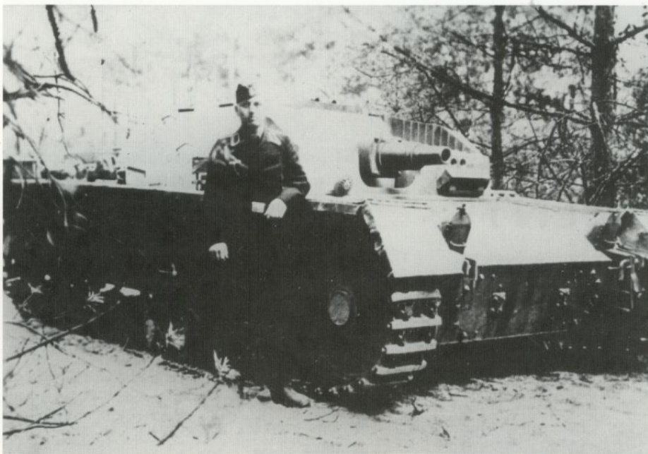
A rare photo of a 's. Pak' from the Veersuchsserie (Experimental Series), which was based on the chassis of the Pz.Kpfw.III Ausf.B. Five such vehicles with soft steel superstructures were built and used for training at the Artillerie Lehr Regiment in Jüterbog. (Chamberlain)
