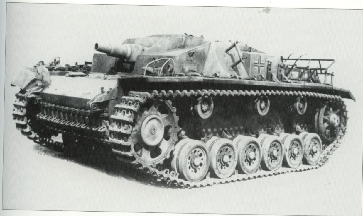
This front three-quarter view of Sturmgeschütz Ausf. D (Fgst. Nr. 90683) shows the driver's visor knocked off by a shell hit. The racks and spare roadwheel mounts were added by the unit. The circular straps over the side intakes are mounts for special pre-cleaning air filters, which gave additional protection to the engine in dusty conditions. (Tank Museum)
