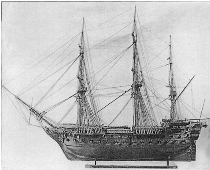
A model of a 74-gun ship of the Surveyor's class (or Vengeur class), a series of 40 ships-of-the-line launched between 1809 and 1812. They were popularly known as 'the Forty Thieves'.
