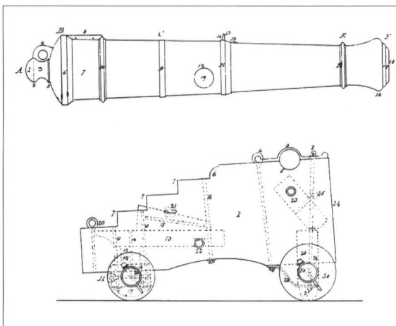
A 24-pdr. long gun of the Blomefield pattern, and its attendant gun carriage. The 'breaching rope' was threaded through the ring above the cascable. (Author's Collection)
