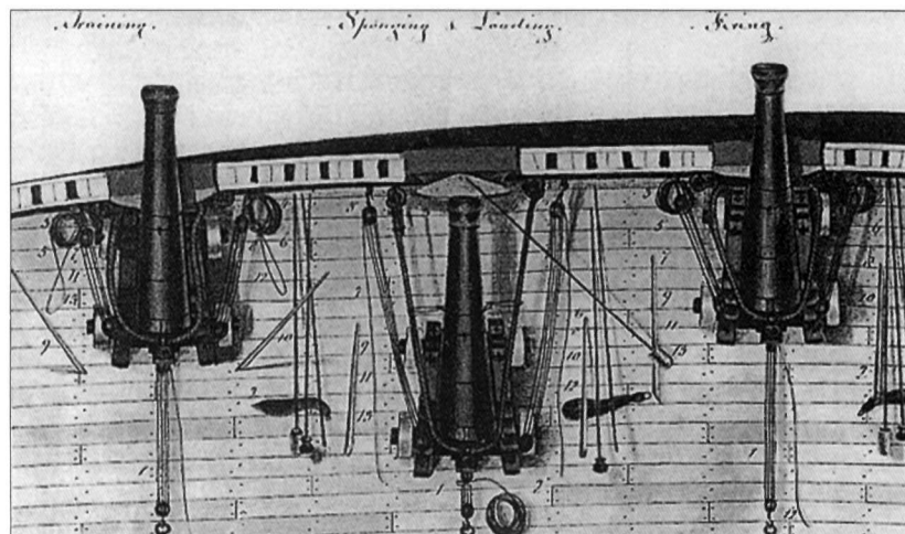
A trio of 12-pdr. long guns mounted on the upper gun deck of a first rate or second rate ship-of-the-line, viewed from above. The illustration clearly shows the arrangement of breeching ropes and pulleys used to move the guns.
