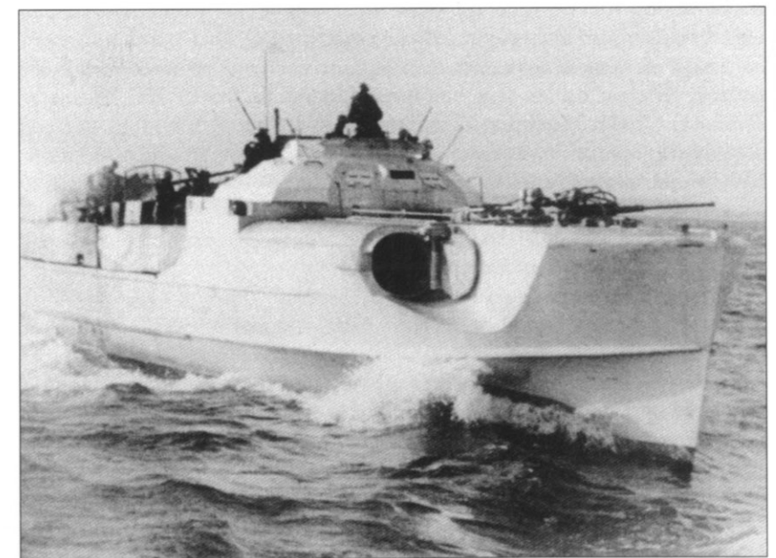
A late-type armoured bridge E-boat. The bow 2cm gun is shown to good effect here, as are the torpedo tube doors. Note also the armoured flaps over the bridge vision ports. The boat does not carry a number on the bow as was normally the case with the training flotillas so it is presumed that this shot may show a boat returning to bay after having expended its torpedoes. Its apparent slow speed certainly does not suggest a boat about to fire its torpedoes during an attack.
