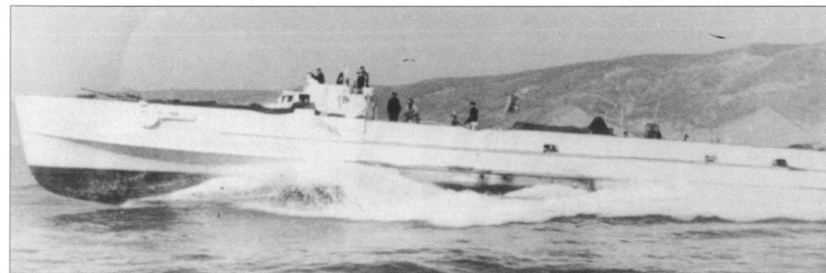
A later high forecastle model moving at speed, its bows raised out of the water to show the black anti-fouling paint used on the lower hull. This model is of the same basic type as those which later had the armoured bridge fitted, as evidenced by the 2cm gun just visible, projecting from its tub on the foredeck. However, it still has the earlier style of open bridge over the wheelhouse. Note that the colour scheme used on most E-boats was a grey so pale that it almost appears white on monochrome photographs.
