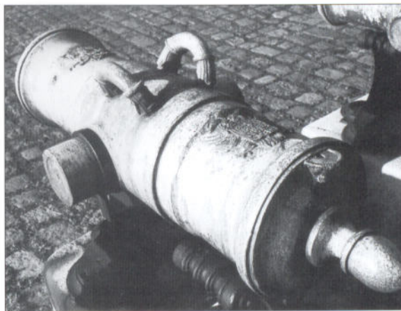
A 7-pdr howitzer barrel. The wider bore extended as far as the rear end of the thicker part.
