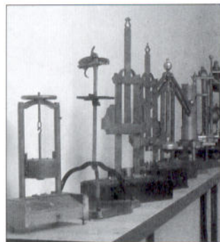
ABOVE From the 18th century, the strength of the powder was tested with a Stangenpulverprobe. In 1812 the French Probemörser with its large bronze counterweight was introduced. Water content was established by drying 100–200 grains at no more than 60 degrees C until they lost no more weight. (Above, Dollezek and below, surviving example)
