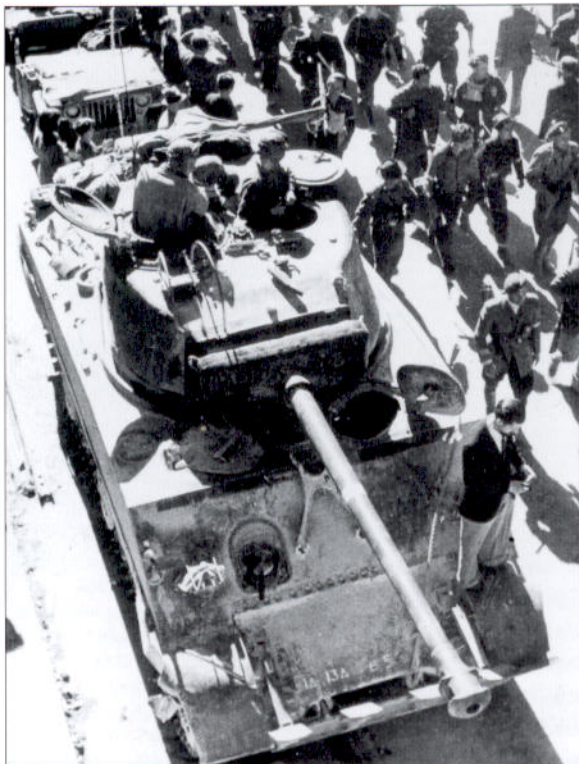
This overhead view of an M4A3 (76mm) of Co. B, 13th Tank Battalion, 1st Armored Division, in Modena, Italy, on April 22, 1945 provides a good view of the features of the late production vehicles from the Grand Blanc tank arsenal with a muzzle brake fitted to the 76mm gun. A new turret casting was introduced in August 1944 which substituted an oval hatch for the loader instead of the previous round split hatch. This tank has the fittings to mount the dozer blade, though it is not attached here. (NARA)
