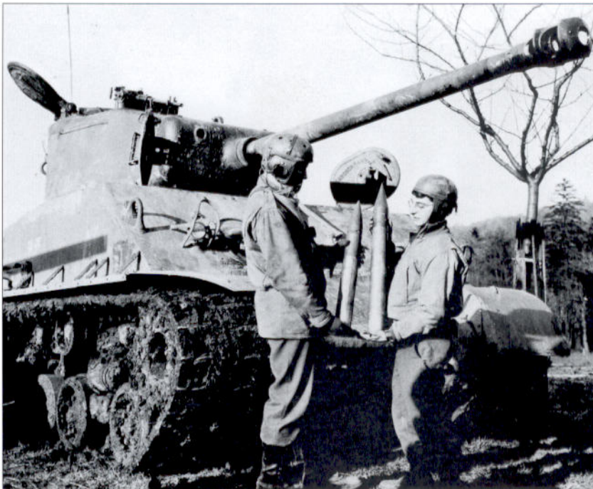
On receiving their new M4A3E8 (76mm) tanks, Co. G, 66th Armored Regiment, 2nd Armored Division, staged a publicity event for army photographers to highlight the new tank. These two tankers show the difference in size between the 75mm ammunition on the left and the 76mm ammunition on the right.
