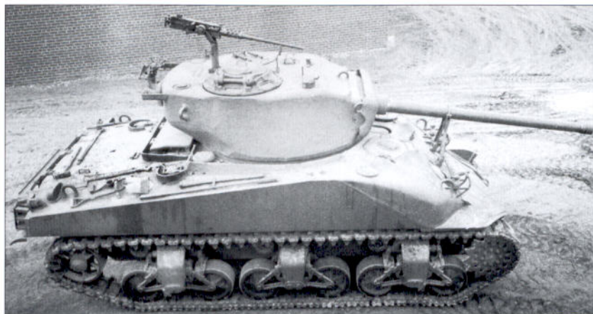
Two pilots of the M4E6 were built, which mated the turret from the new T23 tank to the M4 hull. This is the second pilot, evident from the turret roof which has the oval hatch; the first pilot had a rectangular hatch. This particular vehicle was also fitted with an experimental horizontal volute suspension. (Patton Museum)
