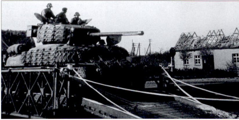
The M4A1 (76mm) (Sherman IIA) was not used by British or other Commonwealth units in northwest Europe, but it was used to re-equip the Polish 1st Armored Division in the late autumn of 1944 when supplies of M4A4 (Sherman V) ran out. This Polish Sherman IIA is seen crossing a Bailey bridge in the Netherlands in 1945, and engineer tape can be seen on either side to mark the mine-cleared areas. The Polish Sherman IIA often had additional track welded to the hull and turret for added protection, and followed the practice used on Sherman Fireflies of camouflage-painting the front of the gun tube so that it would not attract undue attention from German anti-tank gunners. (Sikorski Institute)
