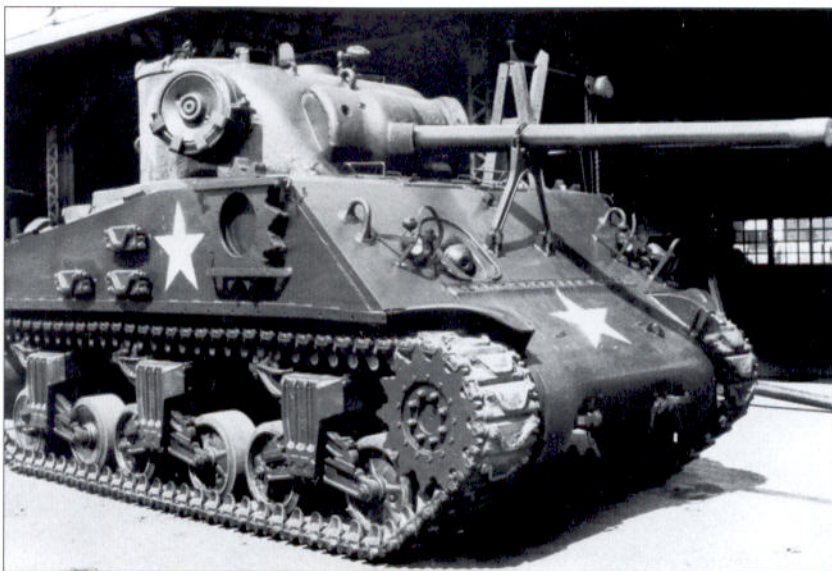
The shortage of M4A3E8 tanks due to post-war scrappings forced the US Army to rebuild many older 75mm M4 tanks to meet the needs of allies. This resulted in the M4A3E4 (76mm) seen here shortly after rebuilding, which mounted the 76mm gun in the standard M34A1 combination gun mount. (US Army)
