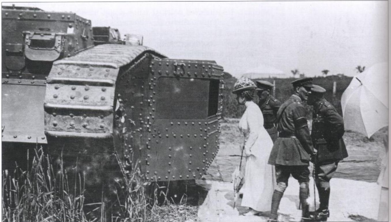
Queen Mary gazes into the blanked-off sponson of a Mark II supply tank. This is a good point to examine the rivet pattern along the top of the cab, which is a distinguishing feature of Mark II and III machines. This inspection took place at Neuve Eglise in the summer of 1917.
