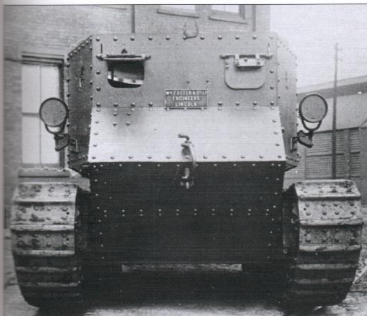
The Lincoln Machine rebuilt as Little Willie . Tritton's new tracks were just 20.5in. (52cm) wide which became standard for all the early tanks. The driver's visor is open, its companion closed and the front machine-gun aperture covered by a round metal plate.
