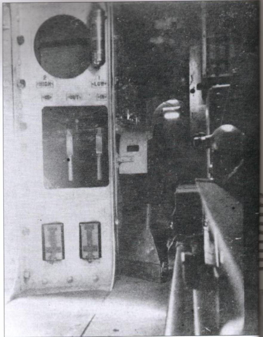
Looking backwards on the right side, the other saddle can just be seen in the glare from the open door. At the centre the starboard auxiliary gear levers hang down, above them another Pyrene extinguisher alongside the gear lubrication tank.
