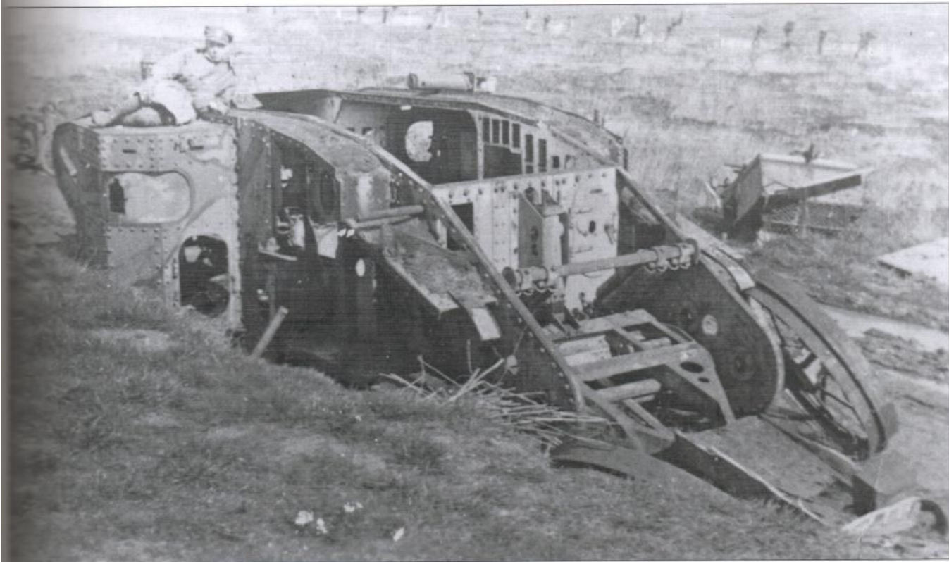
The wreck of D11, photographed much later in the war. Points to note are the vision slits around the top of the sponson, the tail frame with its wooden box, internal stowage for machine-gun ammunition and the spindle for the single top roller. The track skid rails that run along the tops of the frames have been obscured by mud.
