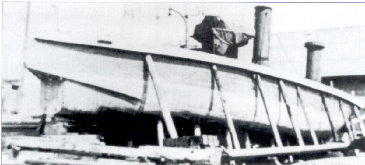
The USS Spuyten Duyvil in the dry dock of Brooklyn Navy Yard after the war. As her bow cutwaters have been removed, the flat plate covering her spar torpedo chamber is clearly visible. (US Naval Historical Center, Washington, DC)
