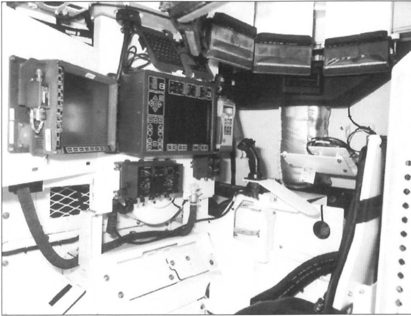
The Stryker vehicle commander's station with the driver's thermal imaging vision enhancer monitor and the Remote Weapons Station's (RWS) Video Display Terminal monitor to the right. Some of the seven M45 periscopes surrounding his overhead hatch can be seen. (GDLS)
