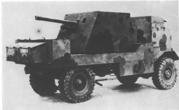
The Deacon, last of the portees. It was outranged even before it entered service. (RAC Tank Museum)
