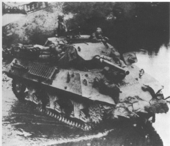
One method of cutting through the banks was by attaching a 'rhino' device, here seen fitted to an M10. The 'rhino' was invented by Sgt. Curtis Culin, US Army, and prevented the vehicle's nose rising as it pushed its way through. Dozer blades were also attached to the M10 and M36. (US Army)
