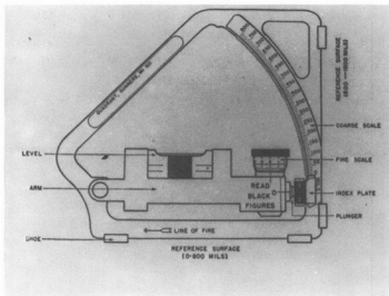
The gunner's quadrant, which, mounted on the breech block and used in conjunction with the traverse indication, permitted tank destroyers to engage in indirect firing.
