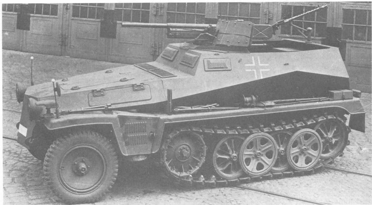
SdKfz 250/10 self-propelled 37mm anti-tank gun mounting; note MG.34 on rear pintle. The 37mm gun was not highly regarded by its users, being termed 'The Military Door-Knocker'. (Bundesarchiv)
